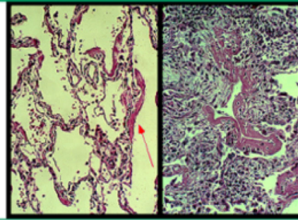
(Left panel) Early changes include diffuse alveolar wall thickening by proliferating connective tissue, type II pneumocytes, and hyaline membranes (red arrow). (Right panel) Later, there is diffuse alveolar wall thickening caused by connective tissue proliferation and inflammation.
